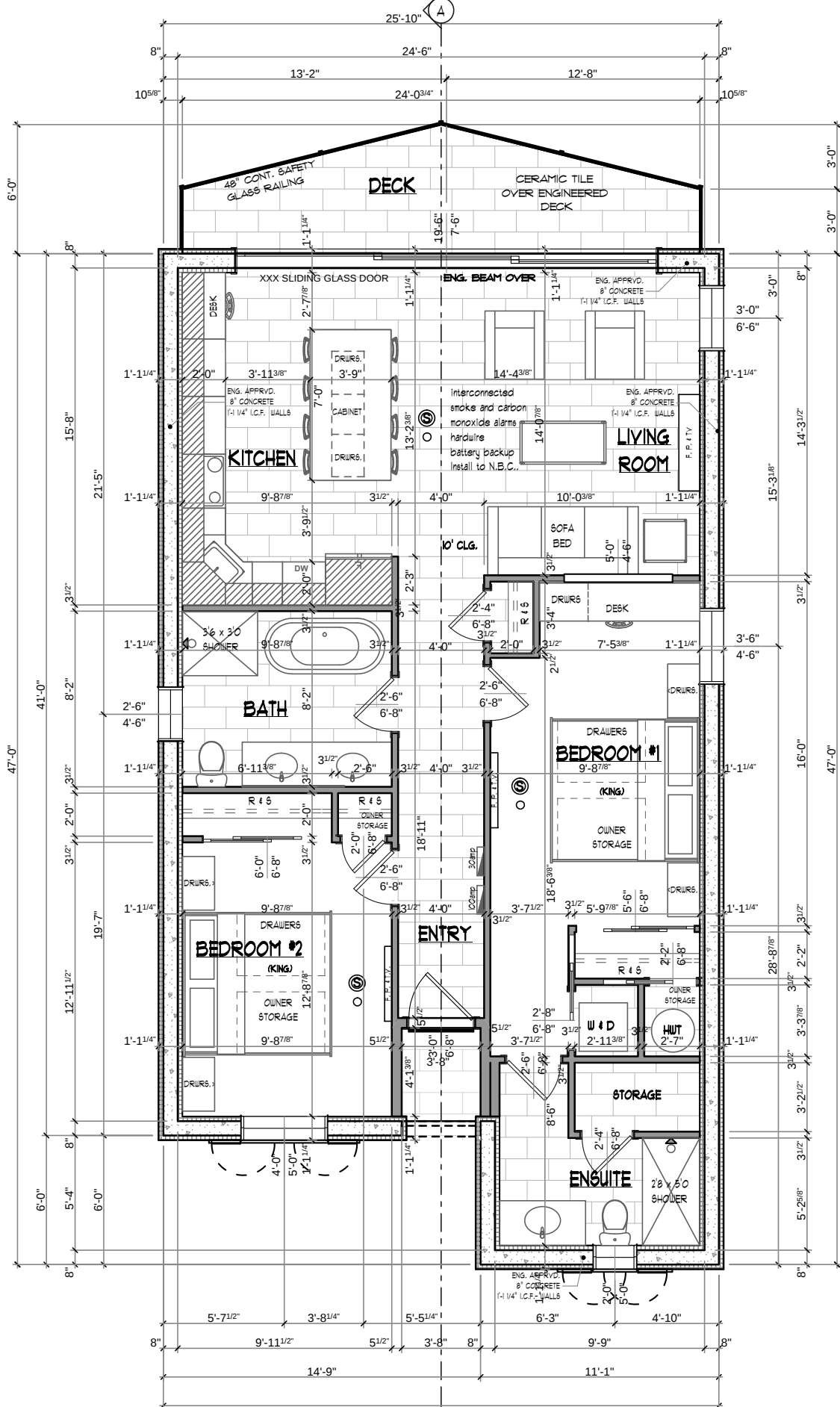
75C MAIN LEVEL PLAN 2BED/2BATH 1107 sq ft
