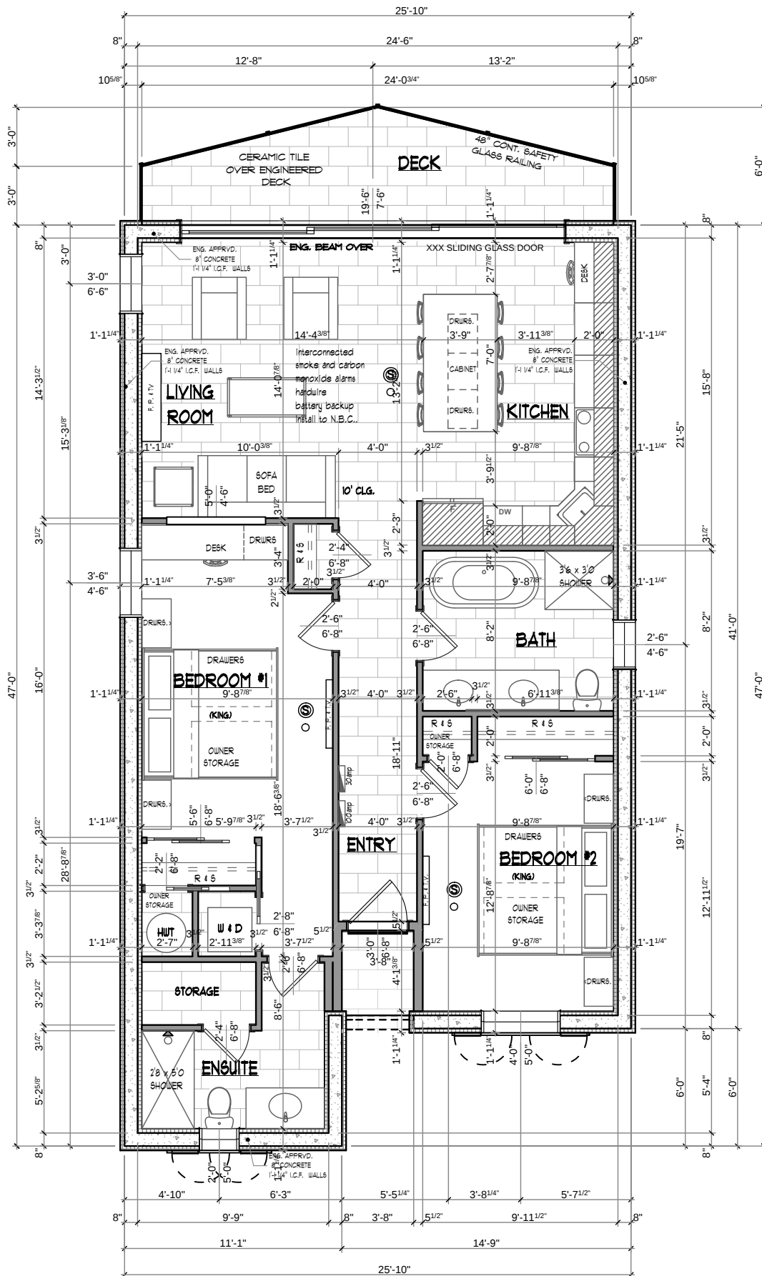
78C MAIN LEVEL PLAN 2BED/2BATH 1107 sq ft
