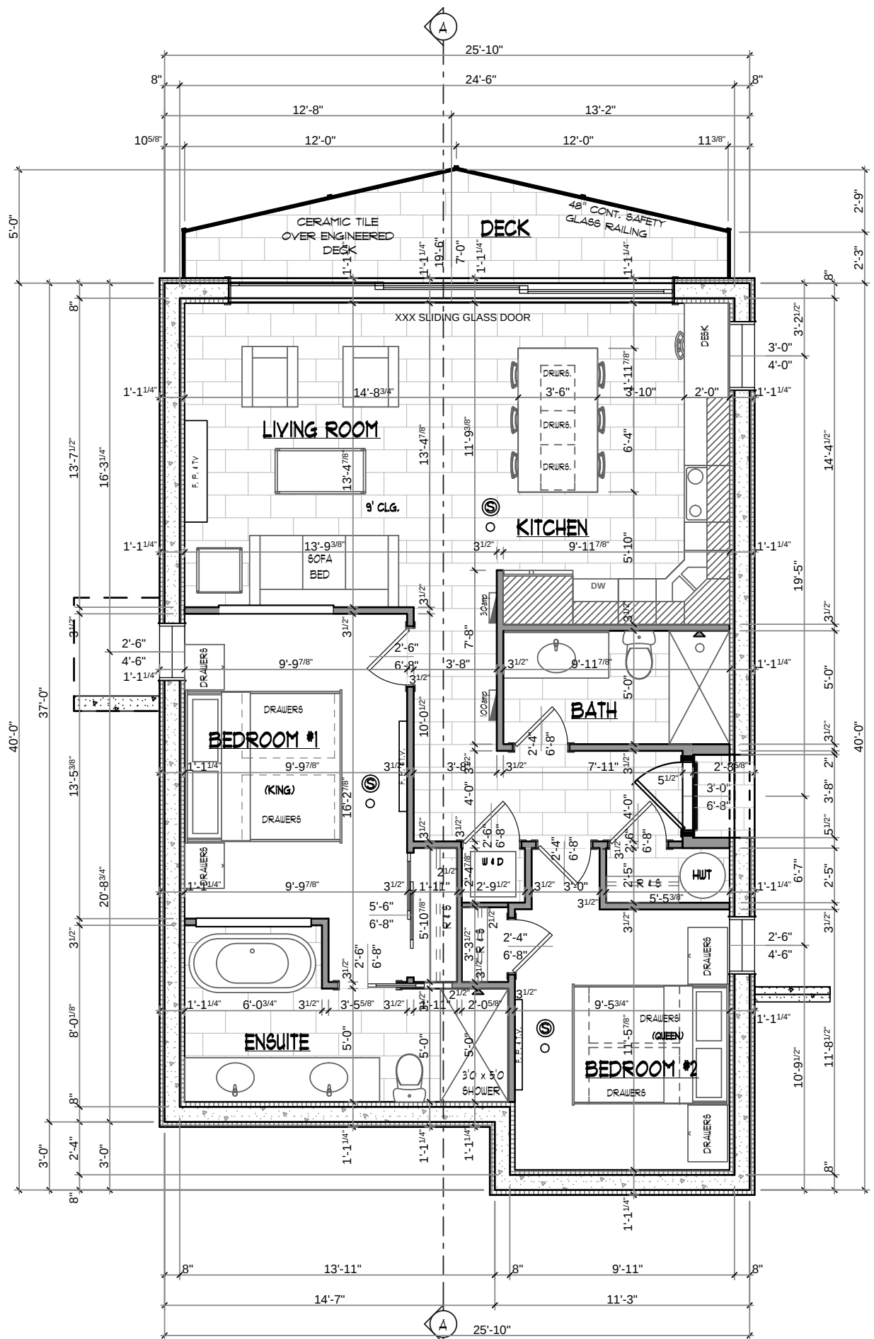
28A LOWER LEVEL PLAN
