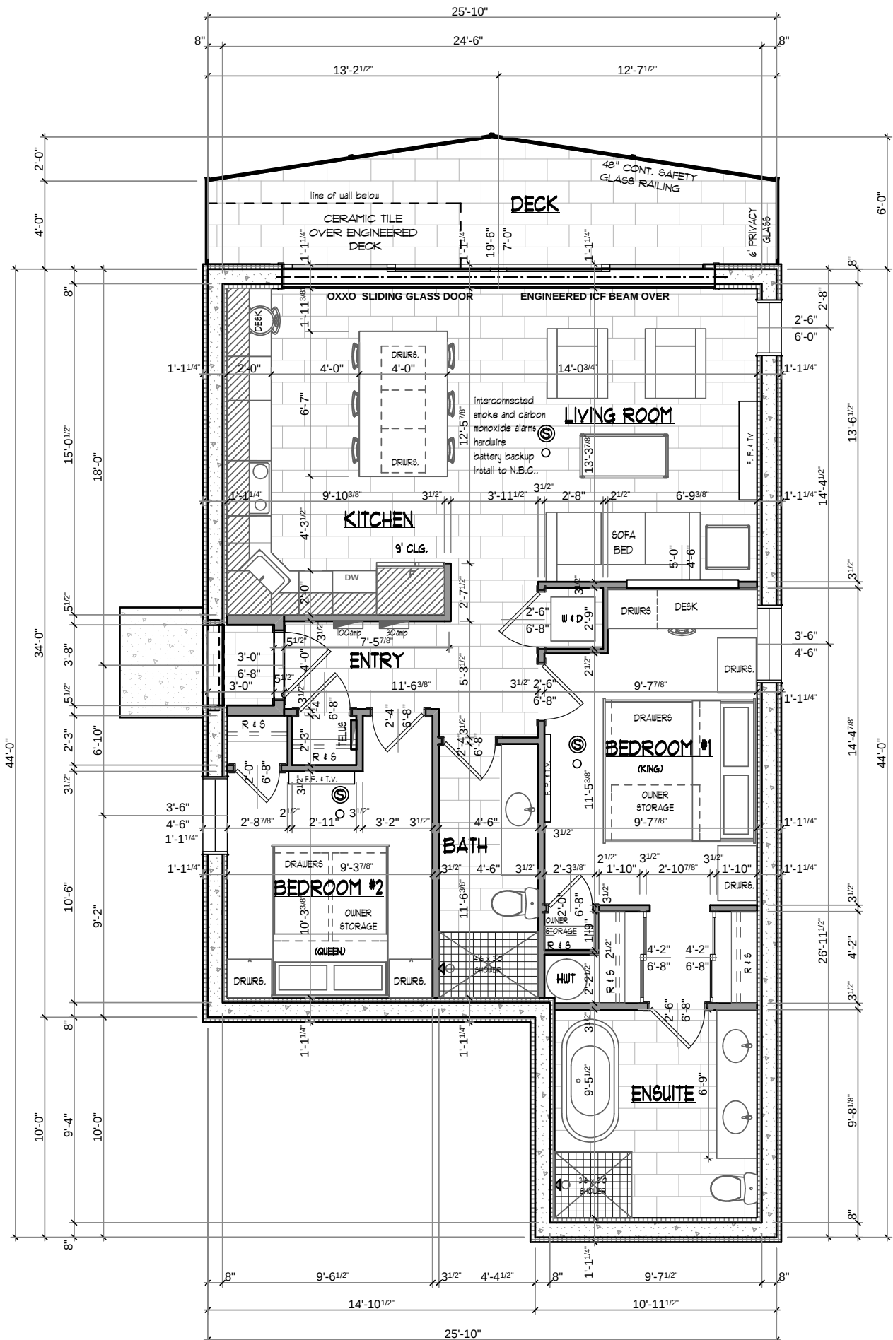
23B MIDDLE PLAN
