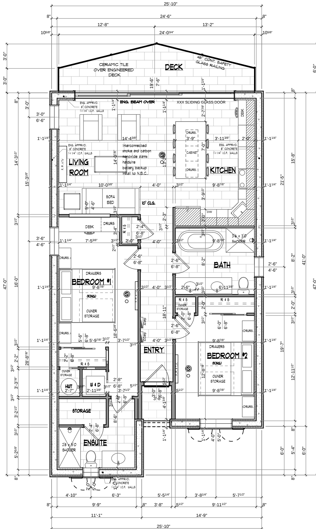
78C MAIN LEVEL PLAN
